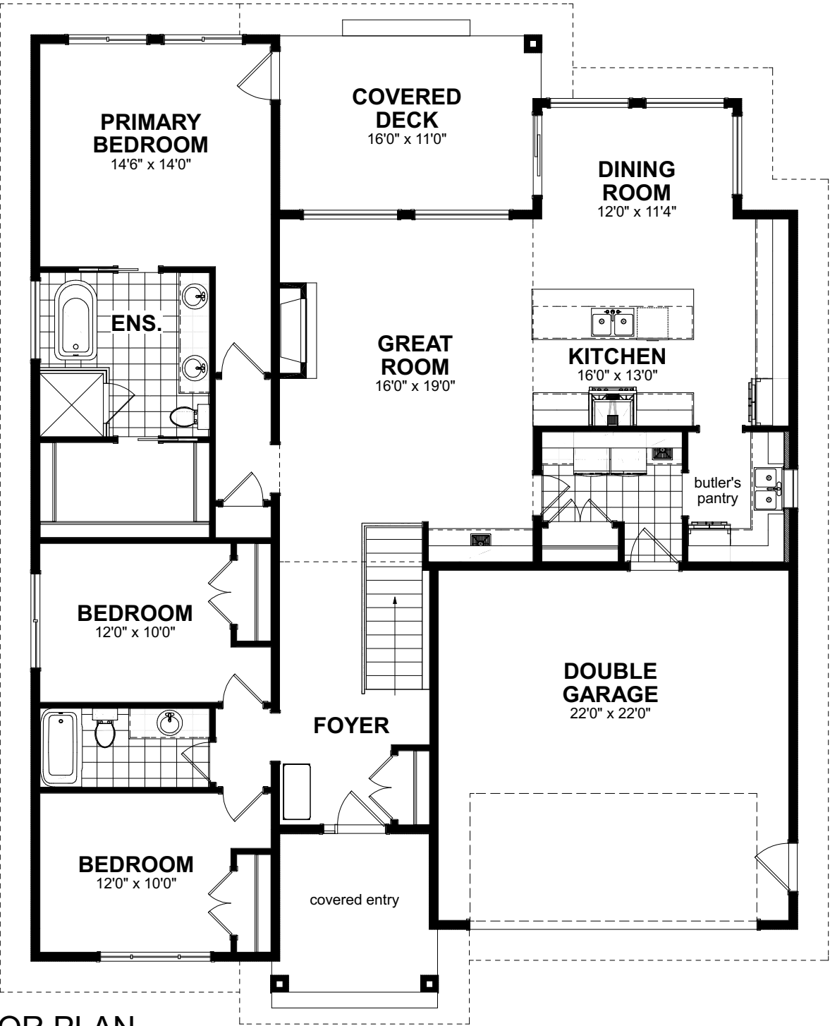
MAIN FLOOR PLAN 1,886 SQ. FT.
