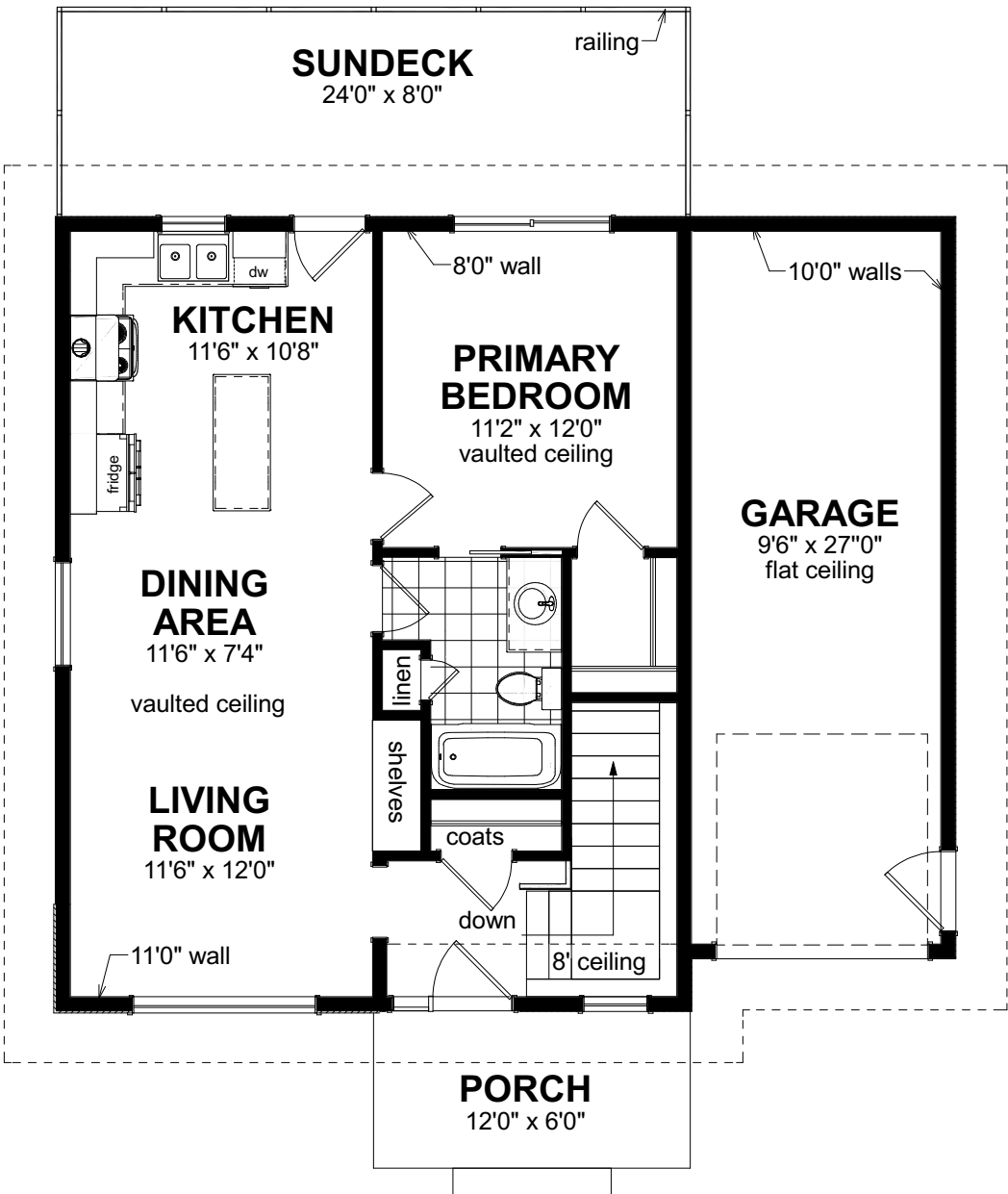
MAIN FLOOR PLAN 720 SQ. FT.
